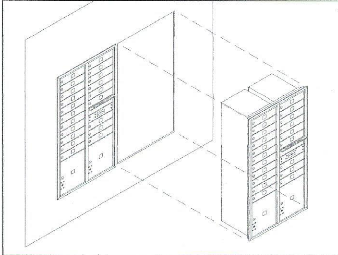
Illustration 1 - Typical Installation
