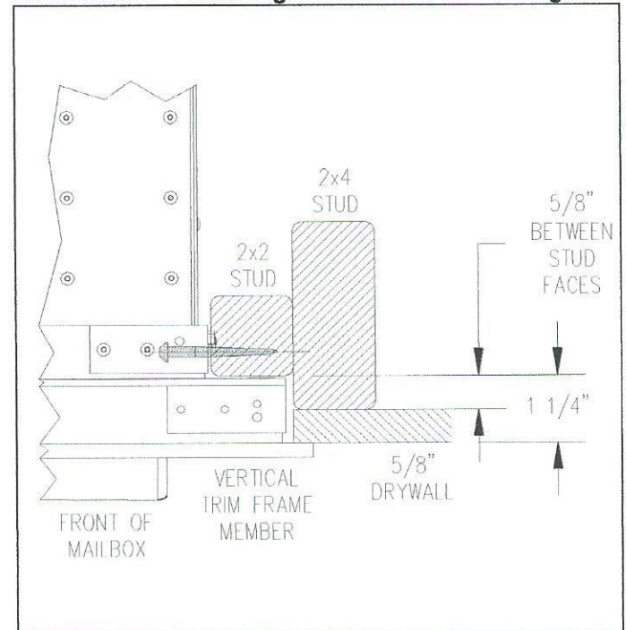
Illustration 2 - Fastening Mailbox Unit to Framing
